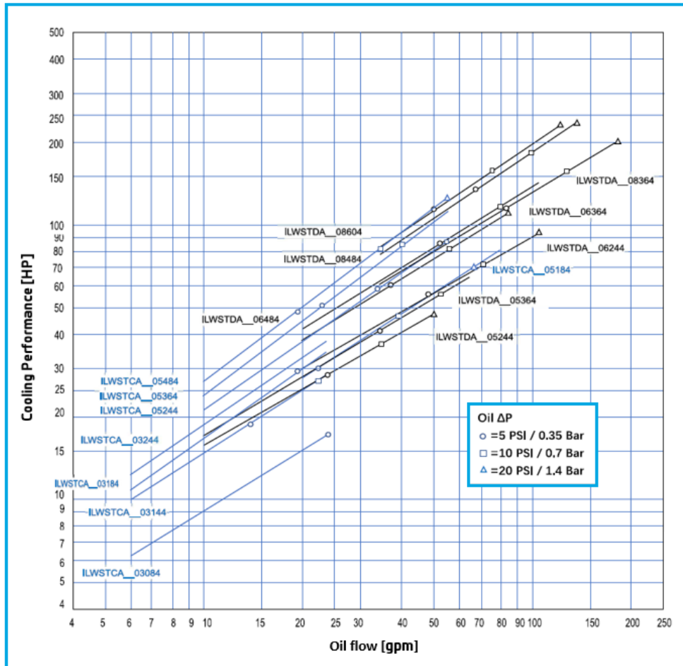
Maximum Water Flow Rates 4 Pass
